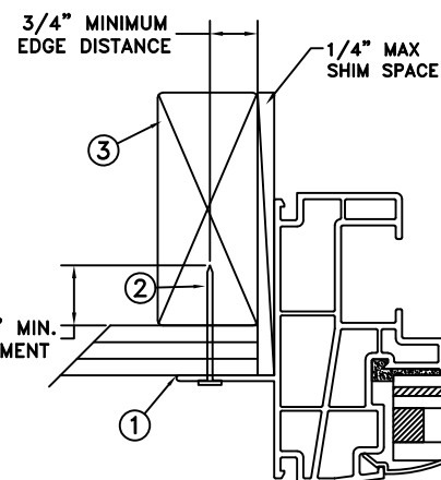
FRAME JAMB SECTION (TYP) HORIZONTAL SECTION
